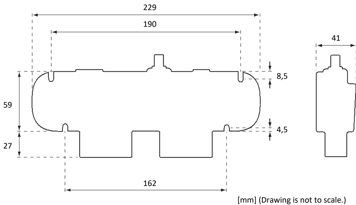
Figure 5.1: Dimensions
