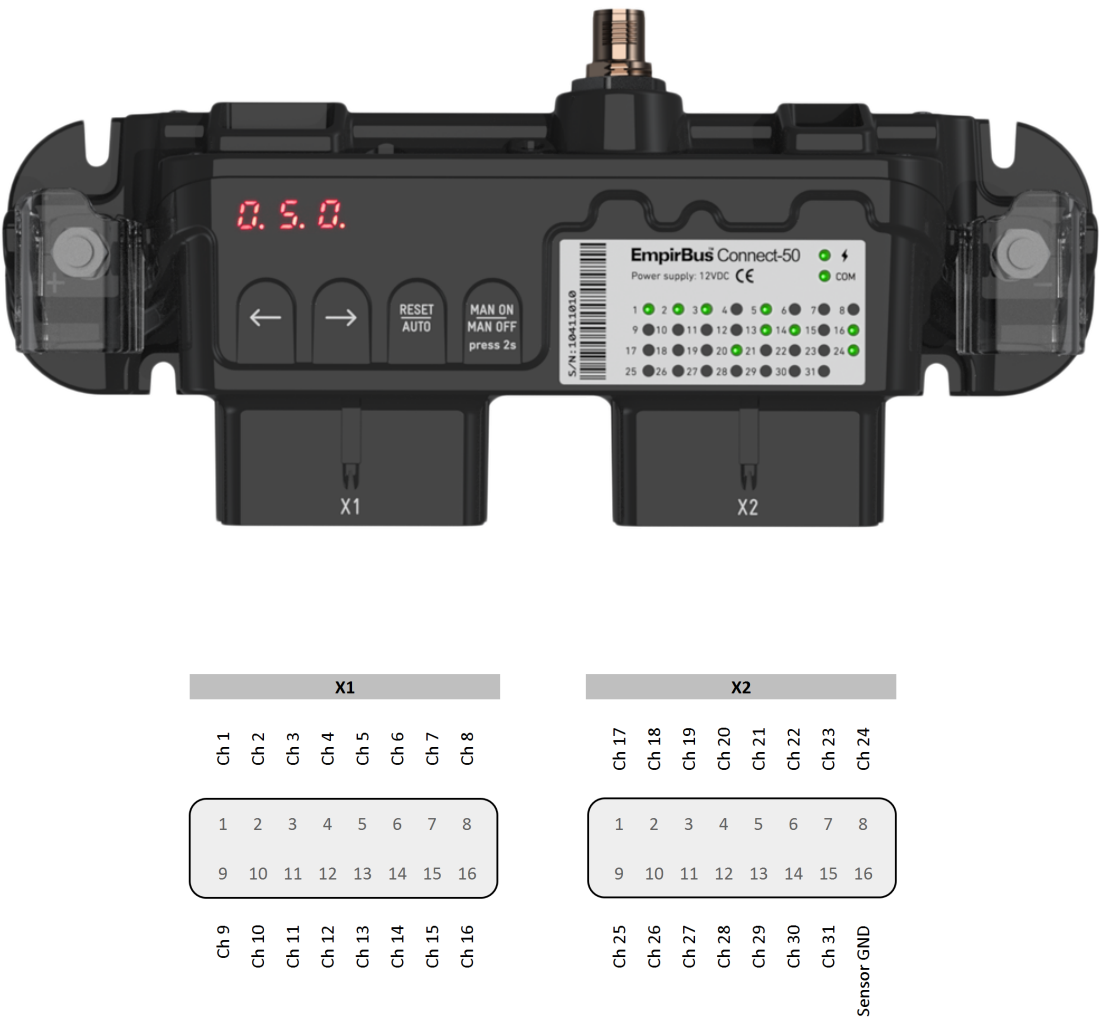
Figure 6.1: pinout
