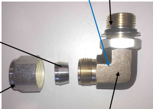
3/4" X 1/2" Tube Fitting Nickel-Bronze Elbow PL-MTE-3/4S1/2B
