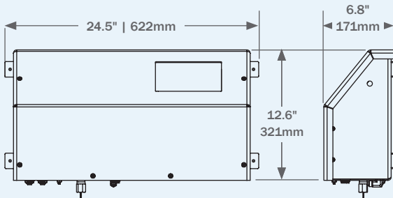
Control Panel
