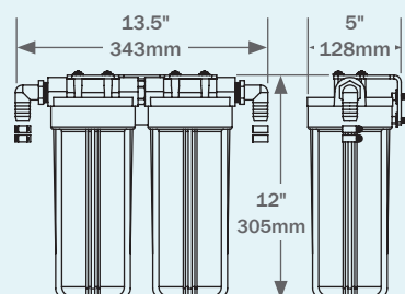
Dual Pre-Filter
