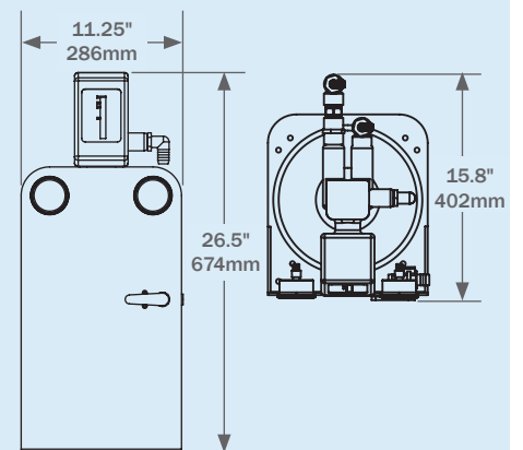
Media Filter
