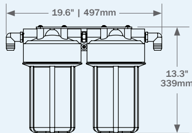
Dual Pre/Post Filter
