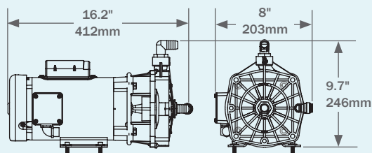
Booster Pump
