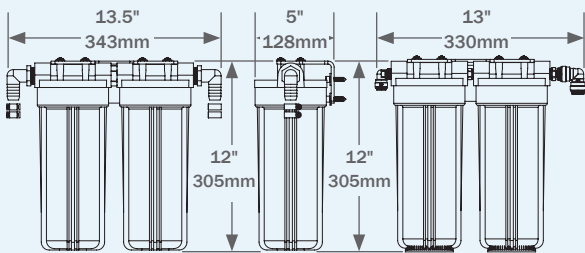
Dual Pre-Filter
