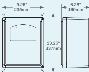
Electric Box
