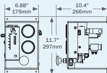
Controller
