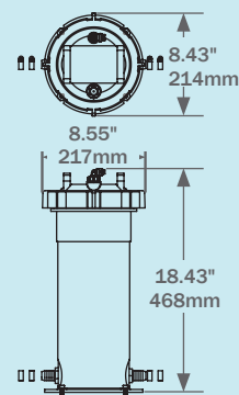
Commercial Pre-Filter / OW Separator
